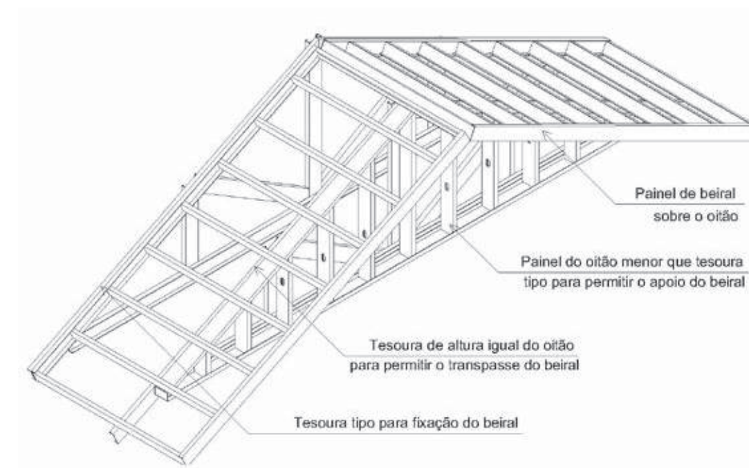
Figura 5.20 - Painel de beiral
